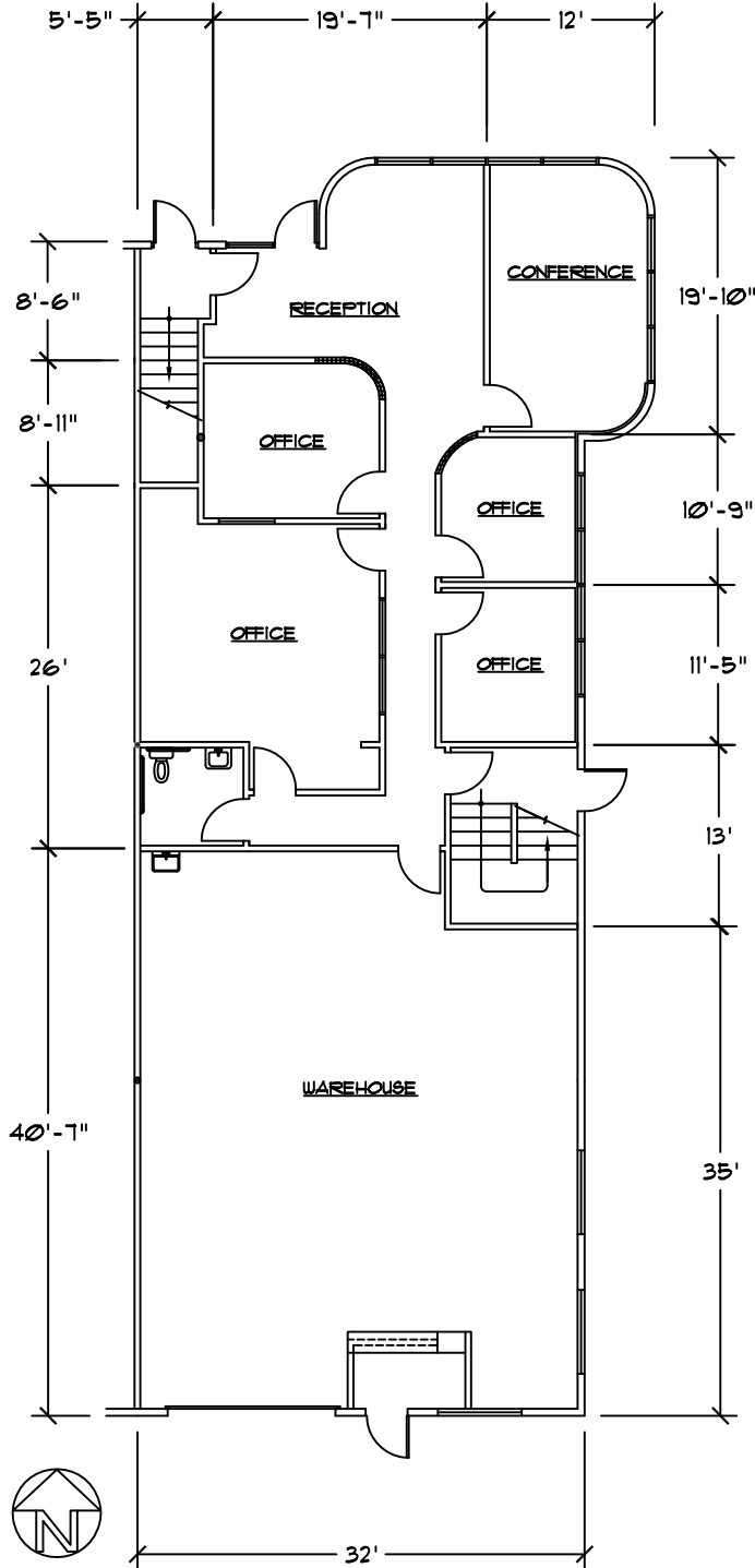
FIRST FLOOR
