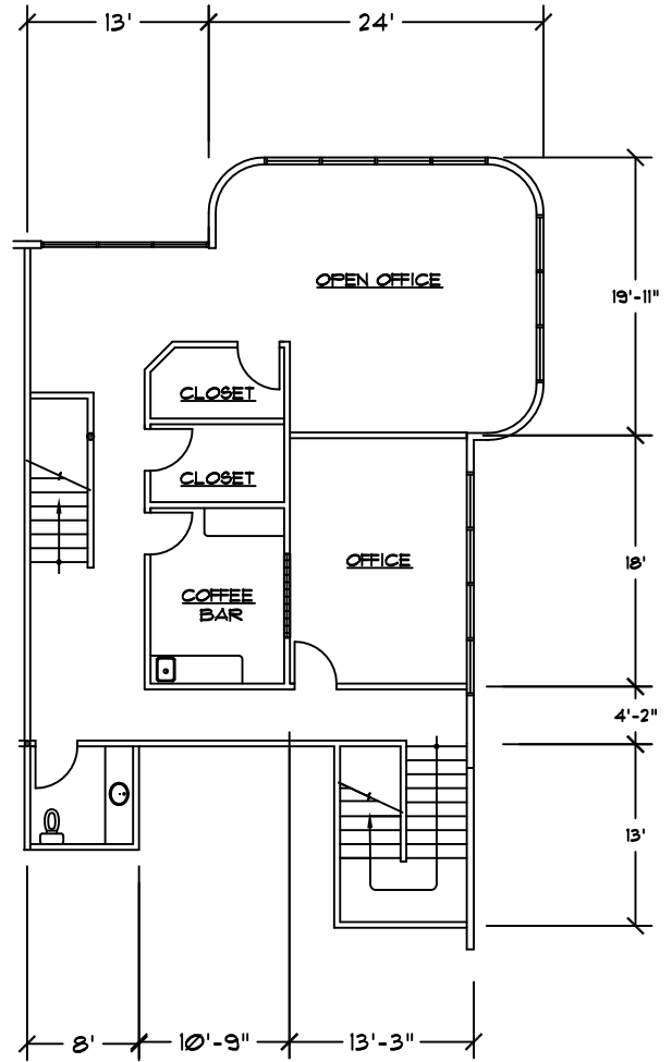
SECOND FLOOR
